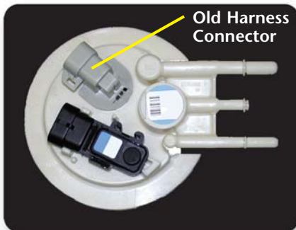
OLD DESIGN-TOP & SIDE VIEW
